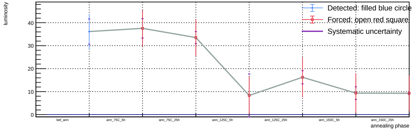
Sensor B1, v = 3\text{ V} , T = 23\text{ }^{\circ}\text{C} - Spot 62: luminosity vs phase
