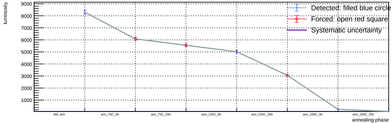
Sensor B1, v = 3 \text{ V} , T = 23 \text{ }^{\circ}\text{C} - Spot 63: luminosity vs phase
