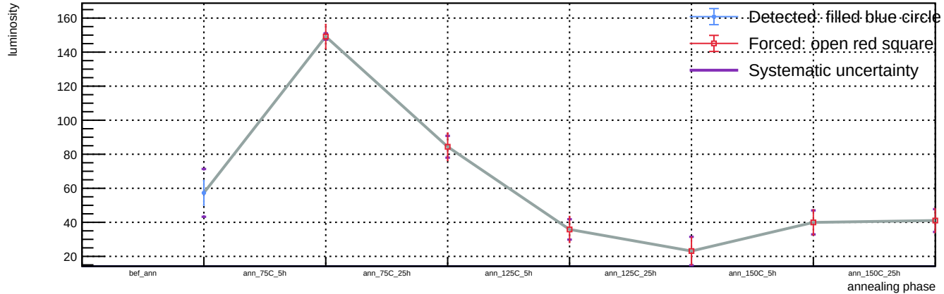
Sensor B1, v = 3 V, T = 23 °C - Spot 64: luminosity vs phase
