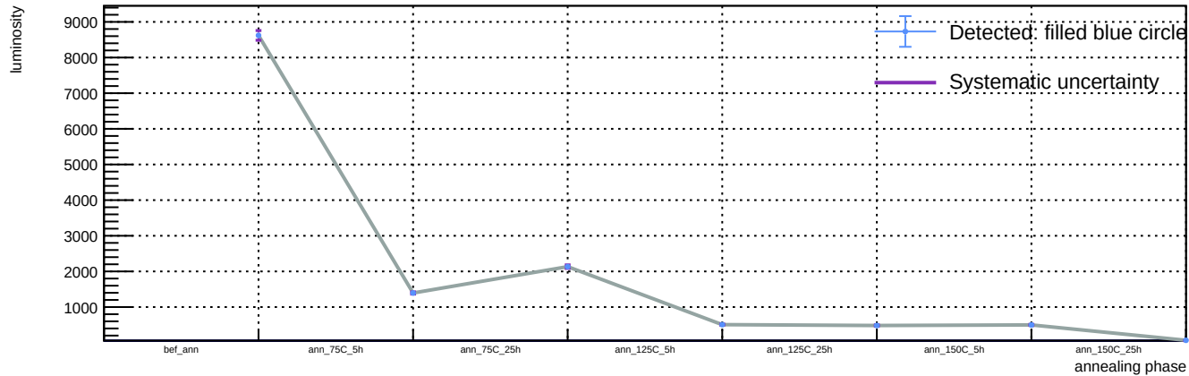
Sensor B1, v = 3 \text{ V} , T = 23 \text{ }^{\circ}\text{C} - Spot 65: luminosity vs phase
