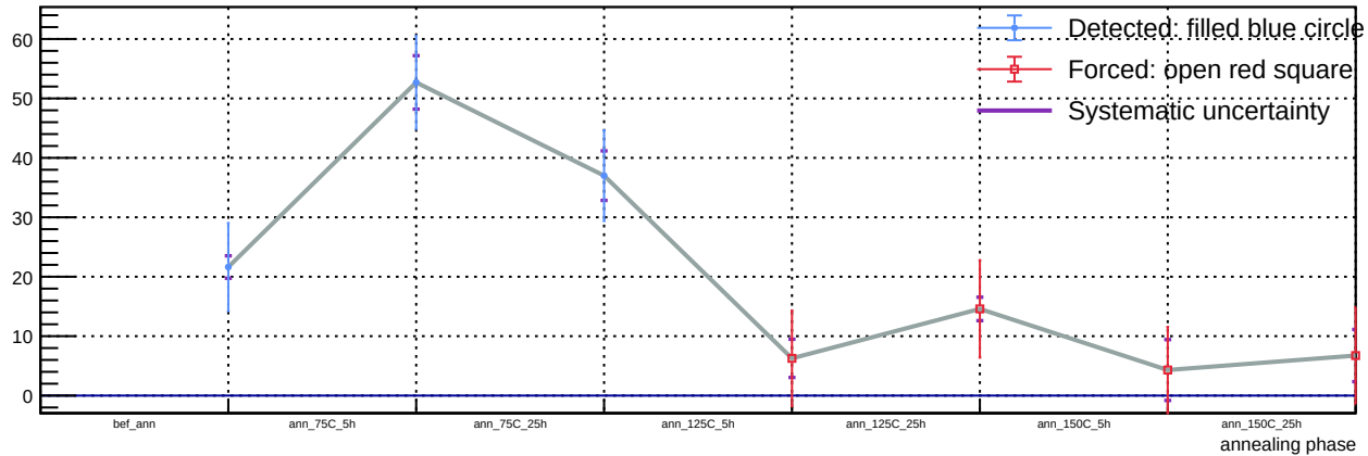
Sensor B1, v = 3 V, T = 23 °C - Spot 66: luminosity vs phase
