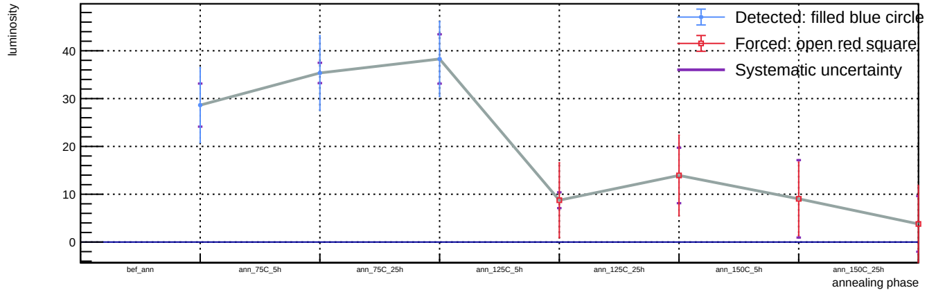
Sensor B1, v = 3\text{ V} , T = 23\text{ }^{\circ}\text{C} - Spot 67: luminosity vs phase
