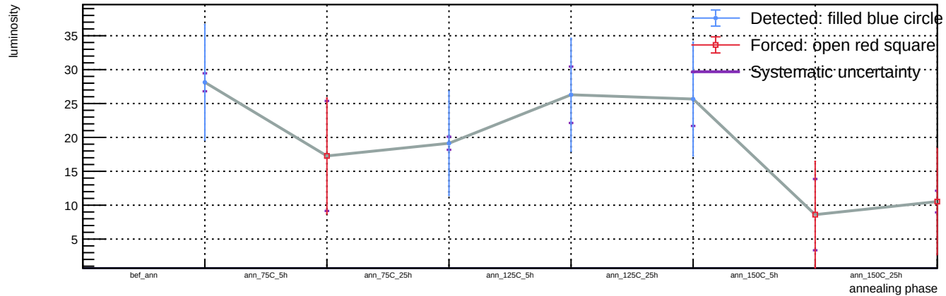
Sensor B1, v = 3 V, T = 23 °C - Spot 68: luminosity vs phase
