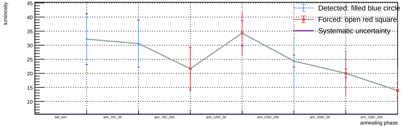
Sensor B1, v = 3\text{ V} , T = 23\text{ }^{\circ}\text{C} - Spot 7: luminosity vs phase
