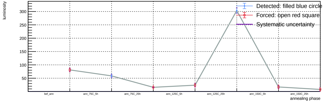
Sensor B1, v = 3 V, T = 23 °C - Spot 70: luminosity vs phase
