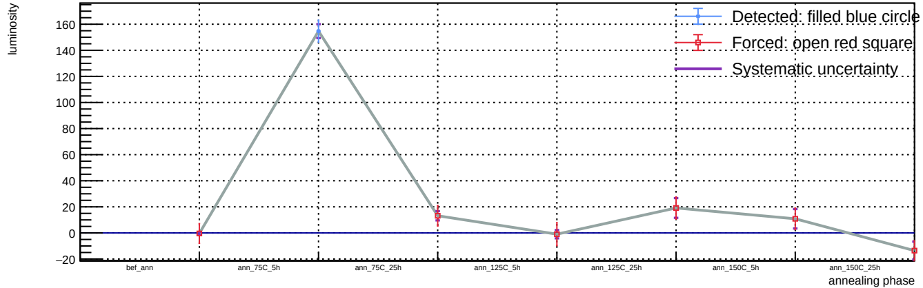
Sensor B1, v = 3 V, T = 23 °C - Spot 71: luminosity vs phase
