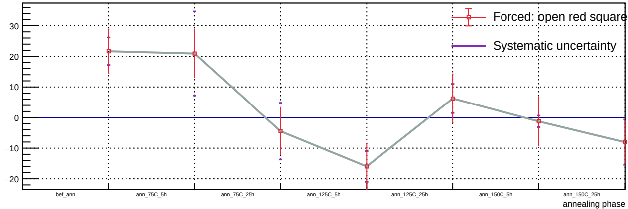
Sensor B1, v = 3 V, T = 23 °C - Spot 72: luminosity vs phase
