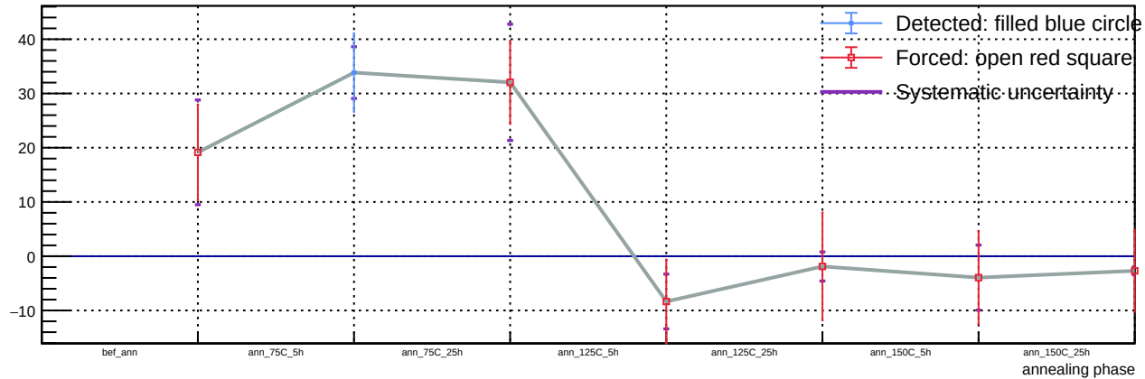
Sensor B1, v = 3 V, T = 23 °C - Spot 73: luminosity vs phase
