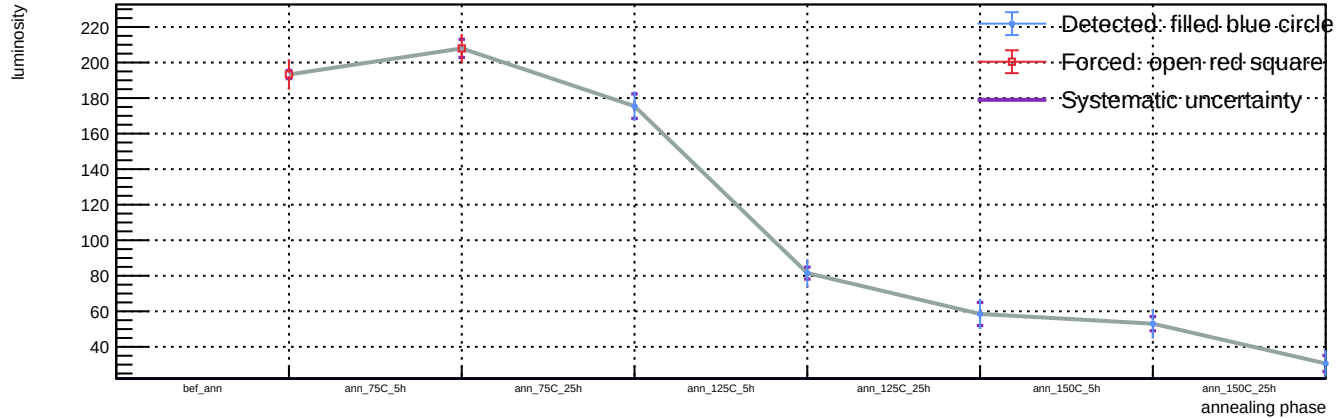
Sensor B1, v = 3 V, T = 23 °C - Spot 74: luminosity vs phase
