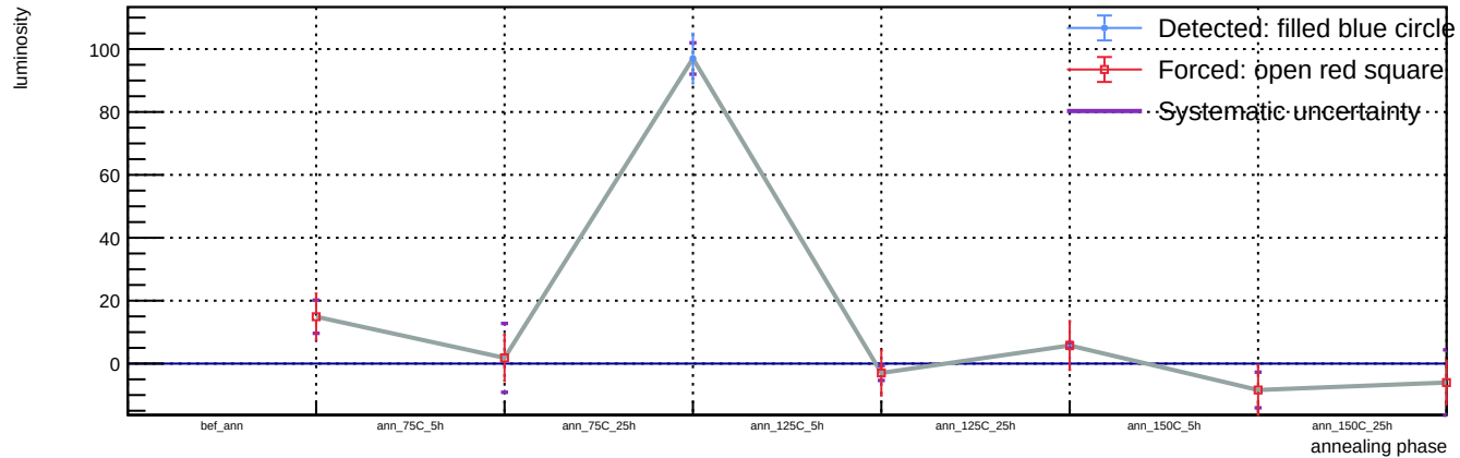
Sensor B1, v = 3 V, T = 23 °C - Spot 76: luminosity vs phase
