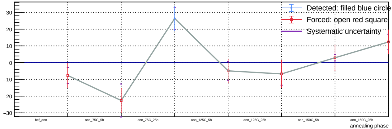
Sensor B1, v = 3 V, T = 23 °C - Spot 77: luminosity vs phase
