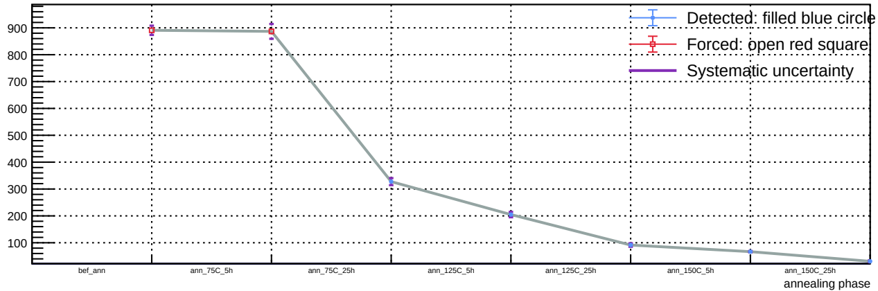
Sensor B1, v = 3 V, T = 23 °C - Spot 78: luminosity vs phase
