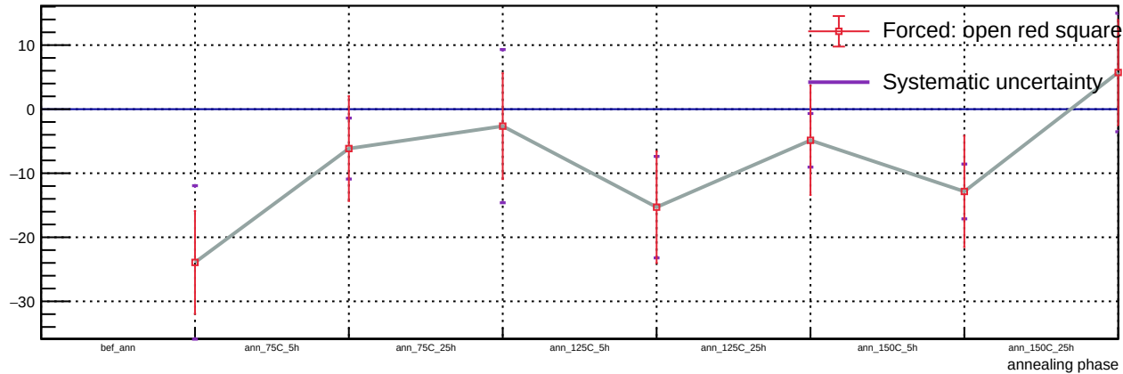
Sensor B1, v = 3 V, T = 23 °C - Spot 79: luminosity vs phase
