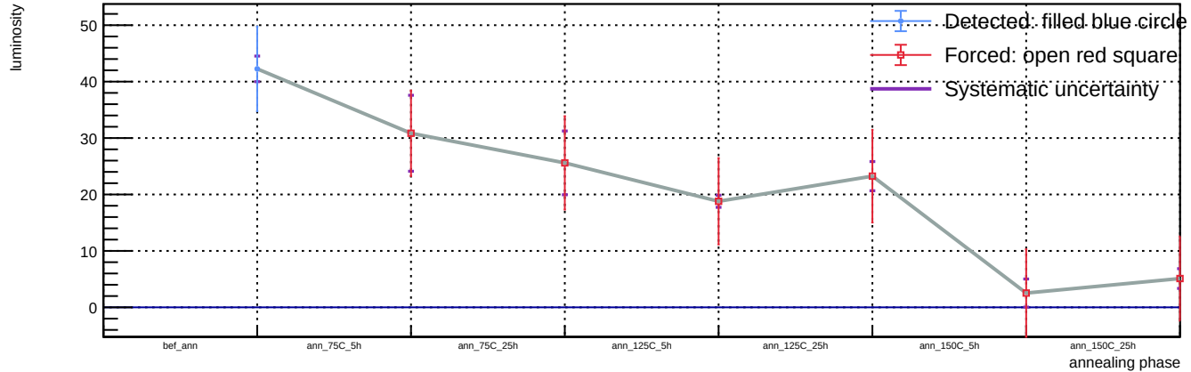
Sensor B1, v = 3 V, T = 23 °C - Spot 8: luminosity vs phase
