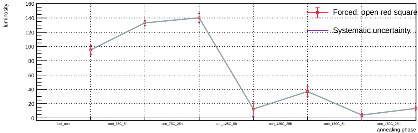
Sensor B1, v = 3 V, T = 23 °C - Spot 80: luminosity vs phase
