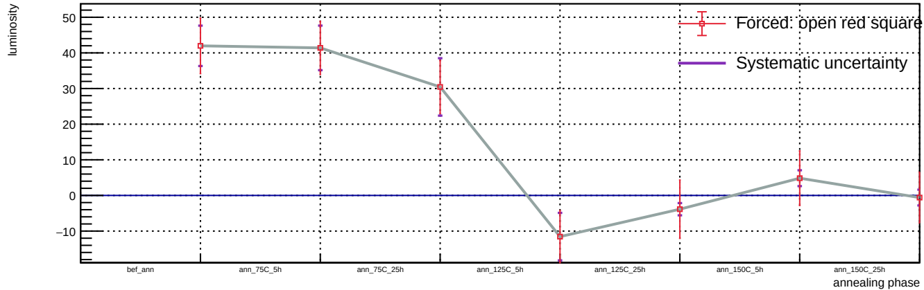
Sensor B1, v = 3 \text{ V} , T = 23 \text{ }^{\circ}\text{C} - Spot 81: luminosity vs phase
