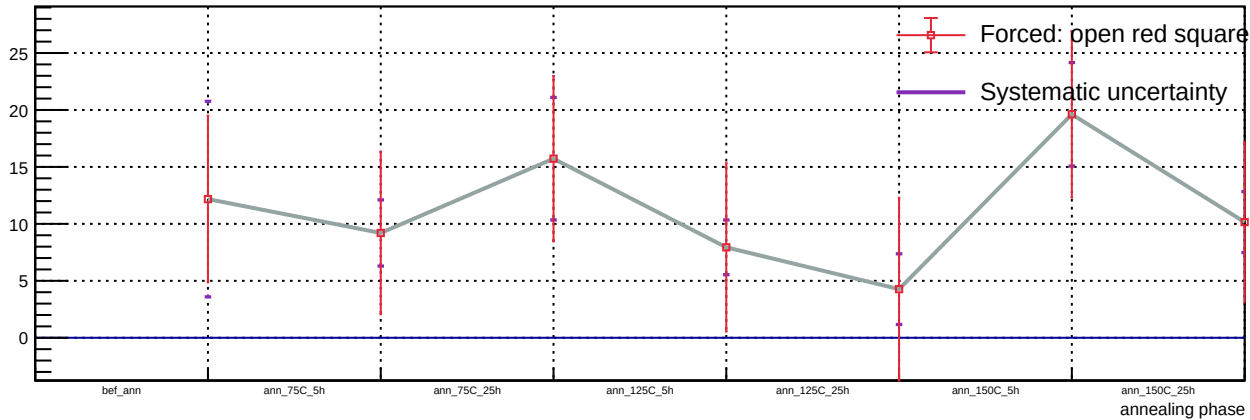
Sensor B1, v = 3 V, T = 23 °C - Spot 82: luminosity vs phase
