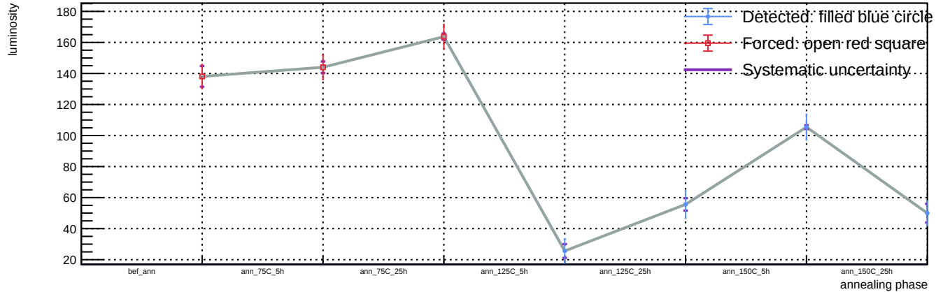
Sensor B1, v = 3 V, T = 23 °C - Spot 83: luminosity vs phase
