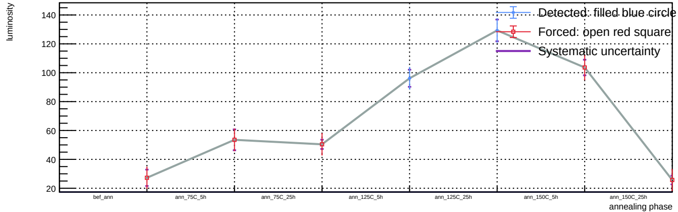
Sensor B1, v = 3 \text{ V} , T = 23 \text{ }^{\circ}\text{C} - Spot 84: luminosity vs phase
