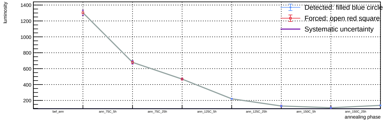
Sensor B1, v = 3 V, T = 23 °C - Spot 85: luminosity vs phase
