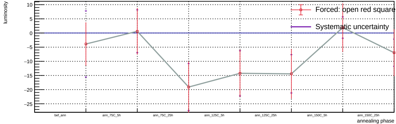
Sensor B1, v = 3 V, T = 23 °C - Spot 86: luminosity vs phase
