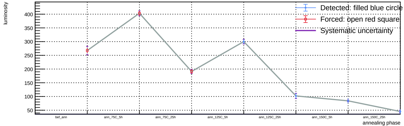
Sensor B1, v = 3 V, T = 23 °C - Spot 87: luminosity vs phase
