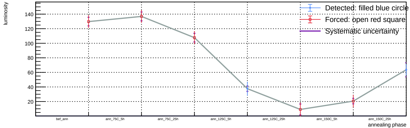
Sensor B1, v = 3 V, T = 23 °C - Spot 88: luminosity vs phase
