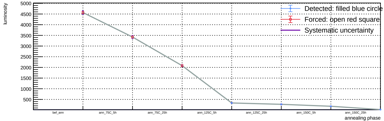
Sensor B1, v = 3 V, T = 23 °C - Spot 89: luminosity vs phase
