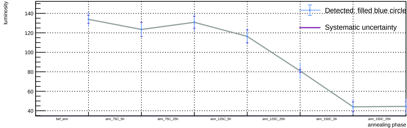
Sensor B1, v = 3 V, T = 23 °C - Spot 9: luminosity vs phase
