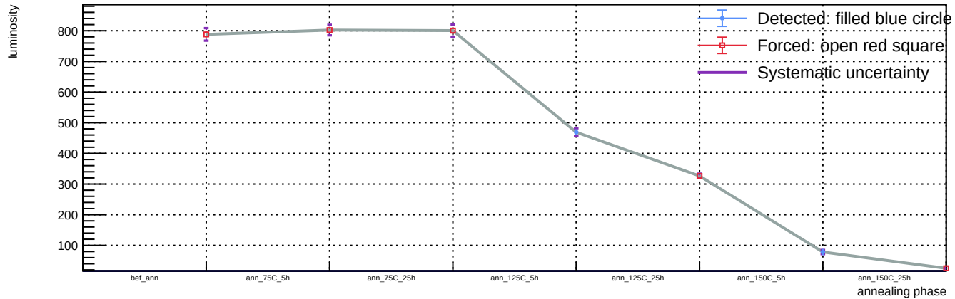
Sensor B1, v = 3 V, T = 23 °C - Spot 90: luminosity vs phase
