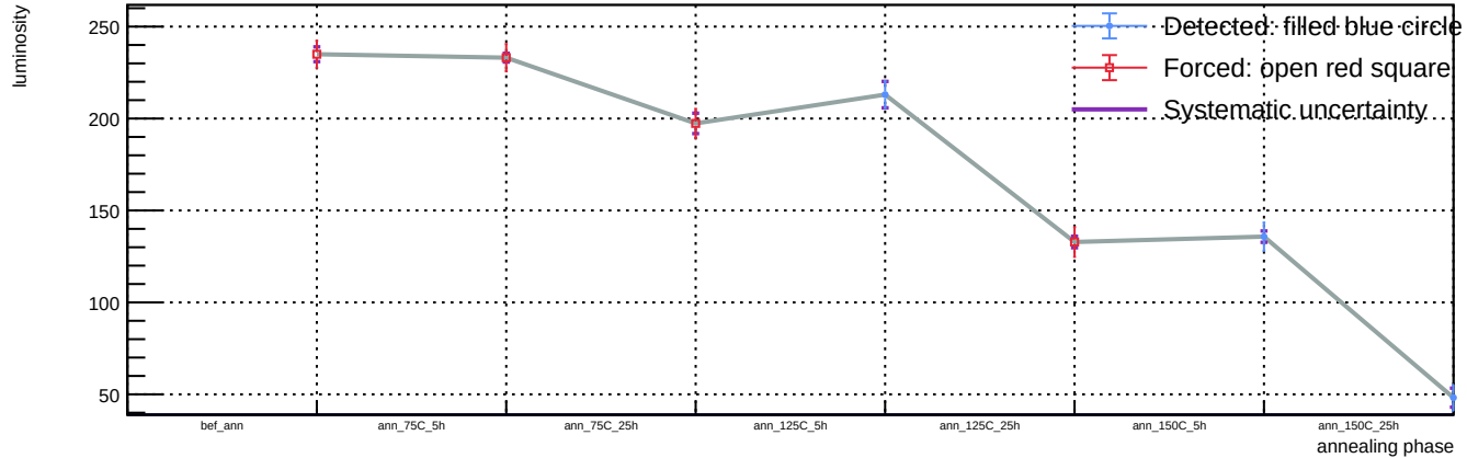
Sensor B1, v = 3 V, T = 23 °C - Spot 91: luminosity vs phase
