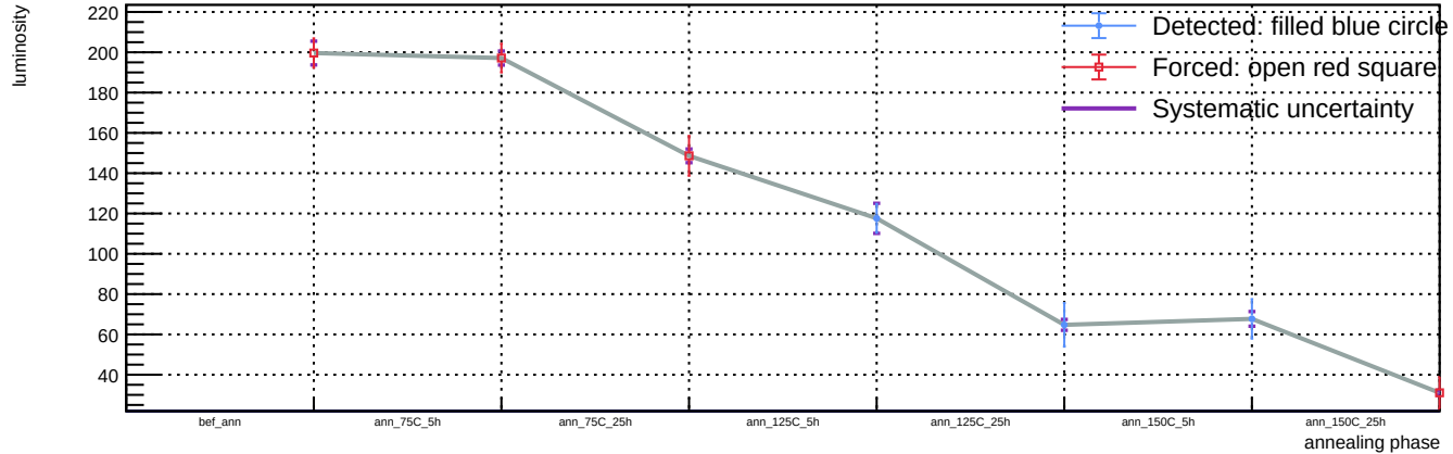
Sensor B1, v = 3 V, T = 23 °C - Spot 92: luminosity vs phase
