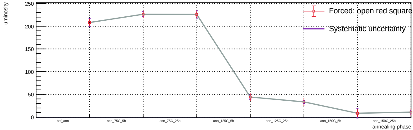
Sensor B1, v = 3 V, T = 23 °C - Spot 93: luminosity vs phase
