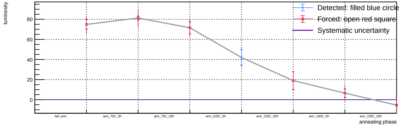
Sensor B1, v = 3 V, T = 23 °C - Spot 95: luminosity vs phase
