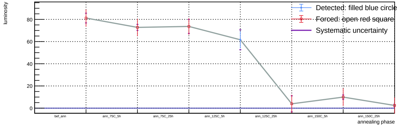
Sensor B1, v = 3 V, T = 23 °C - Spot 96: luminosity vs phase
