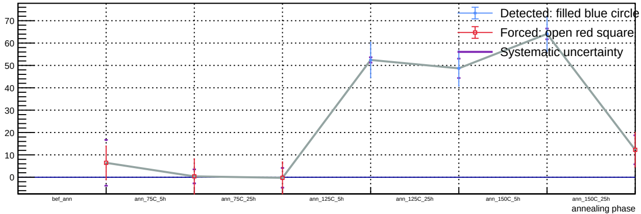
Sensor B1, v = 3 V, T = 23 °C - Spot 98: luminosity vs phase
