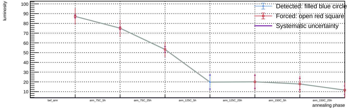
Sensor B1, v = 3 V, T = 23 °C - Spot 99: luminosity vs phase
