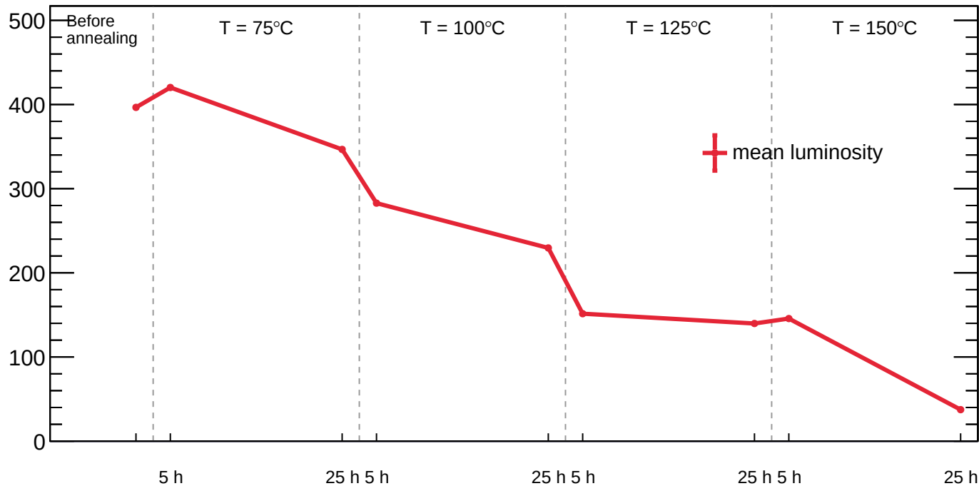
Sensor A1 - Mean luminosity vs annealing phase, T = 20^{\circ}\text{C} , v_{\text{over}} = 5 \text{ V}
