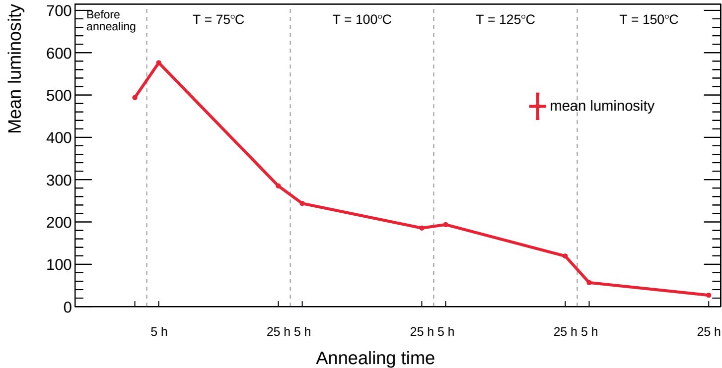
Sensor B1 - Mean luminosity vs annealing phase, T = 20^{\circ}\text{C} , v_{\text{over}} = 3 \text{ V}
