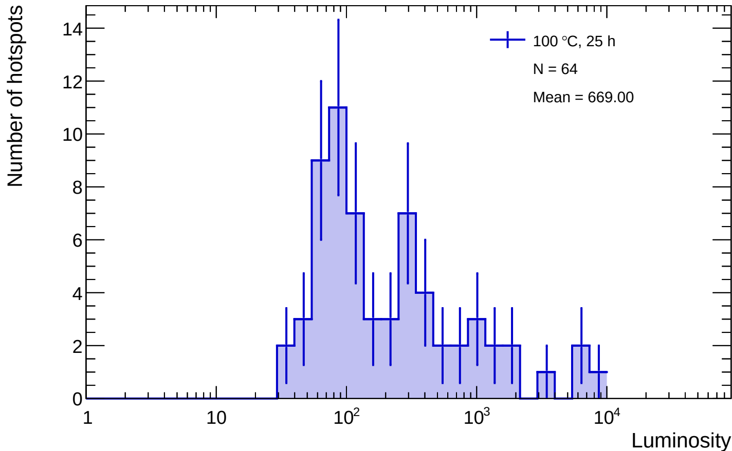
Sensor A1 - 100 °C, 25 h luminosity distribution
