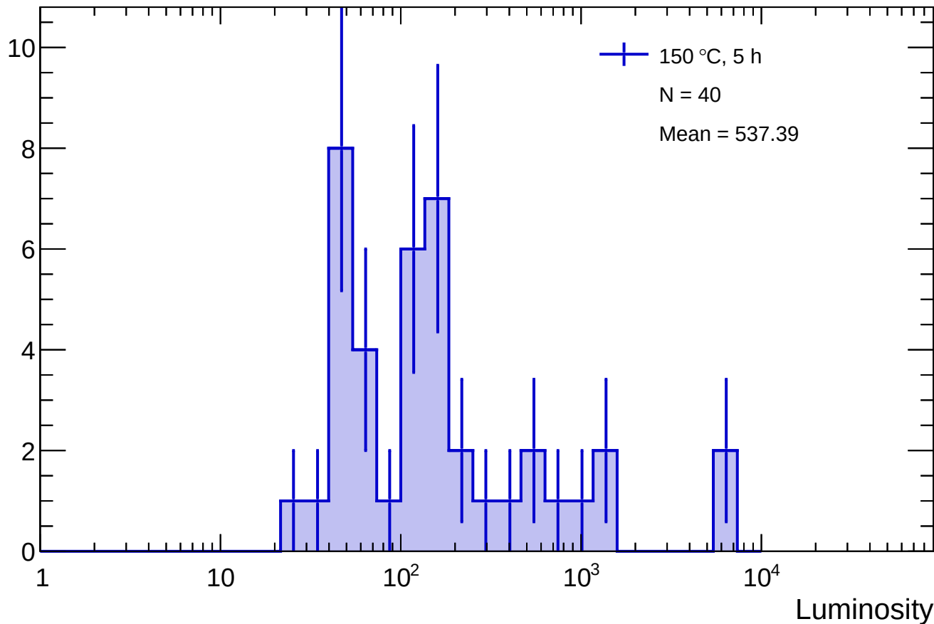
Sensor A1 - 150 °C, 5 h luminosity distribution
