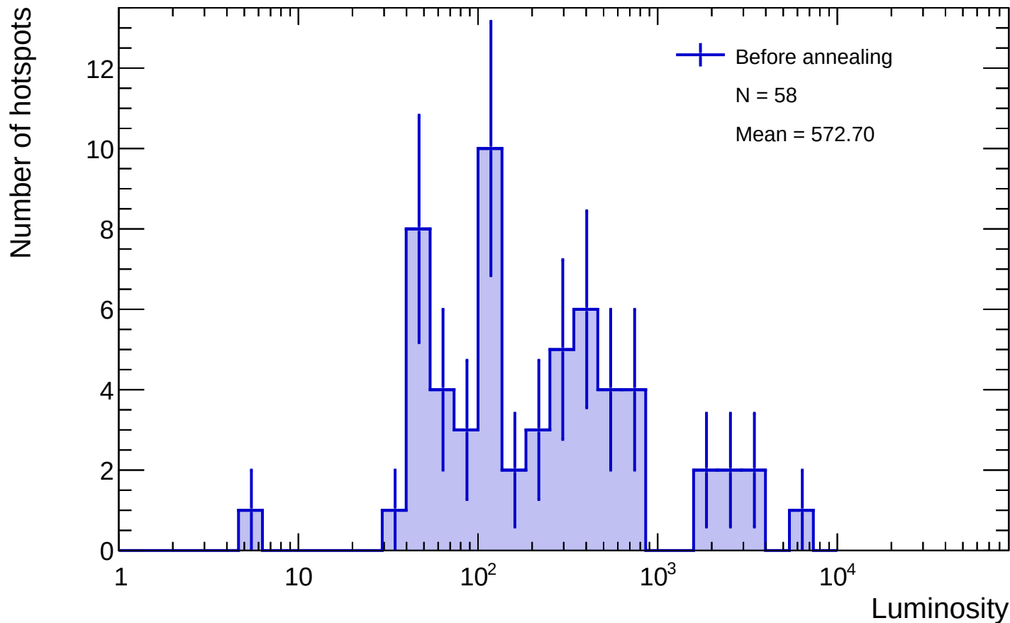
Sensor A1 - Before annealing luminosity distribution
