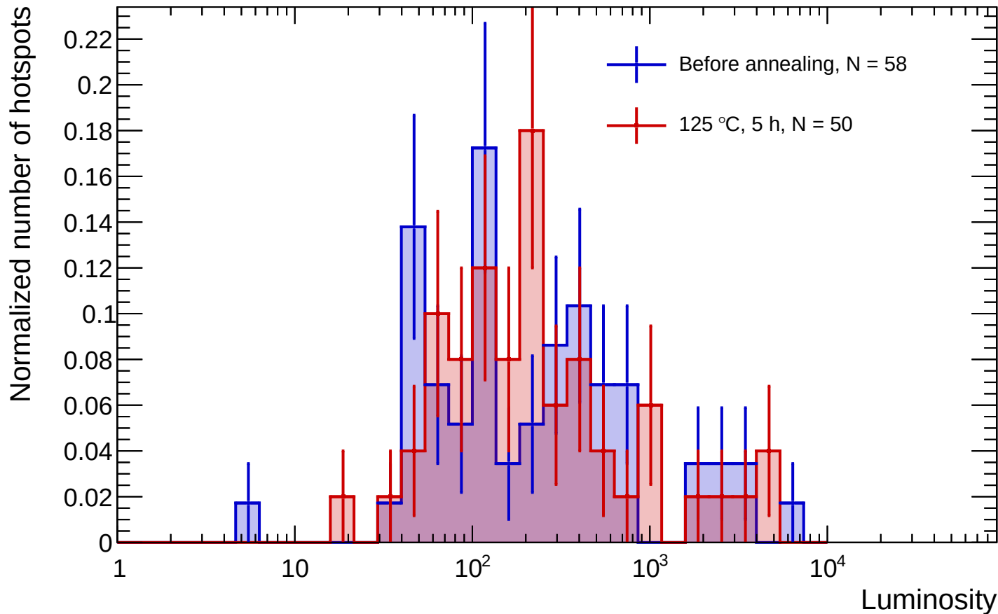
Sensor A1 - Before annealing vs 125 °C, 5 h luminosity distributions
