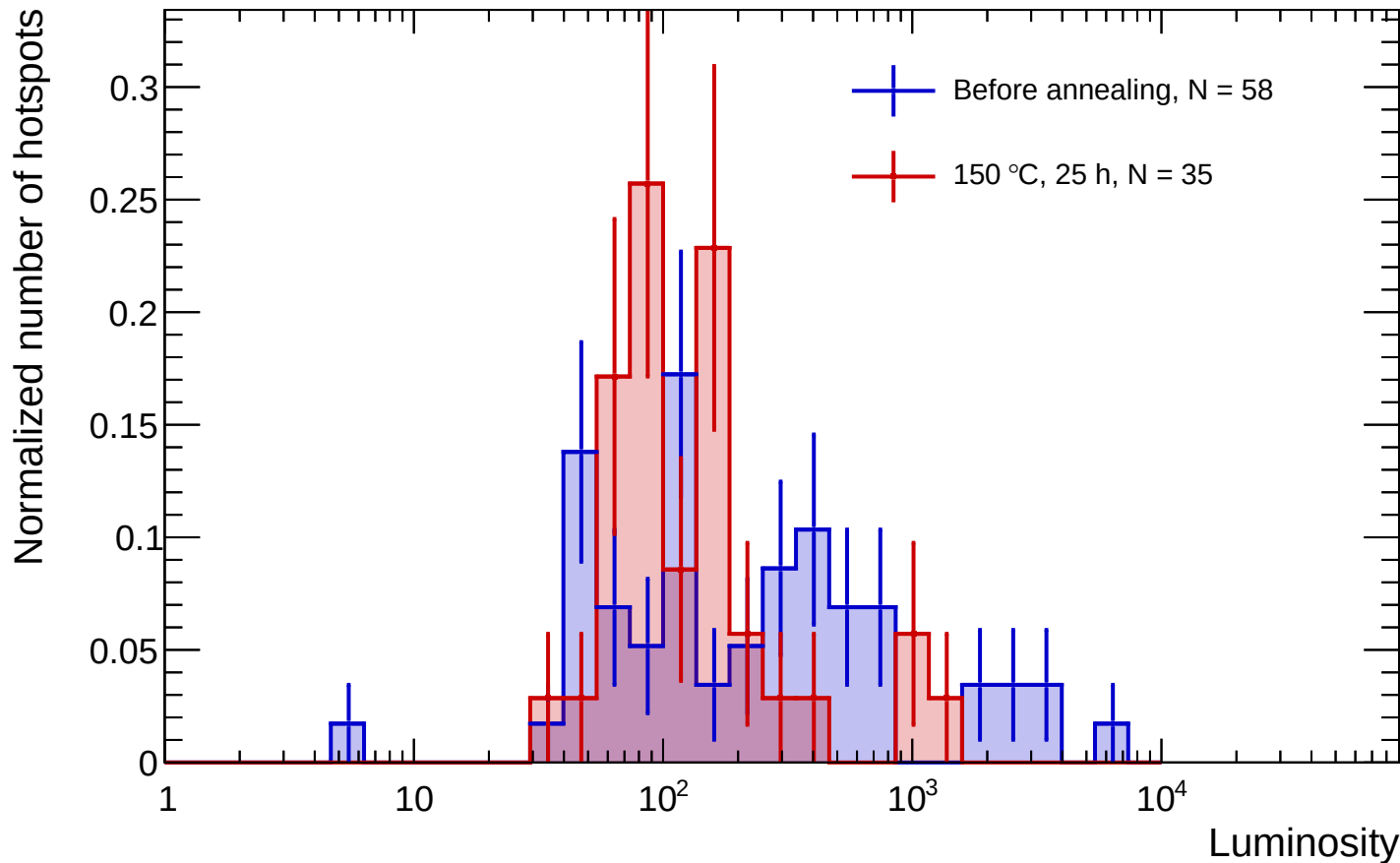
Sensor A1 - Before annealing vs 150 °C, 25 h luminosity distributions
