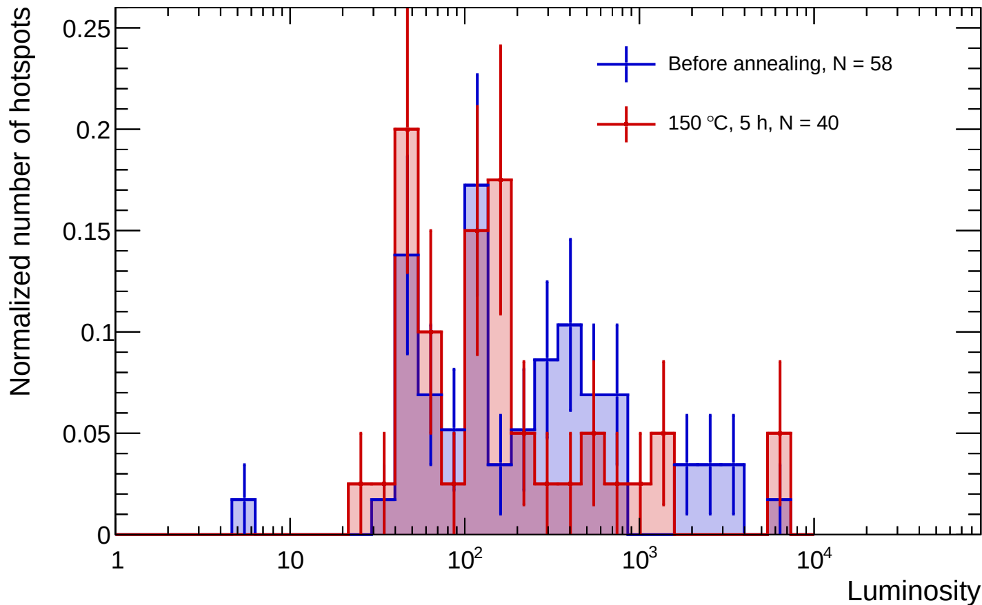
Sensor A1 - Before annealing vs 150 °C, 5 h luminosity distributions
