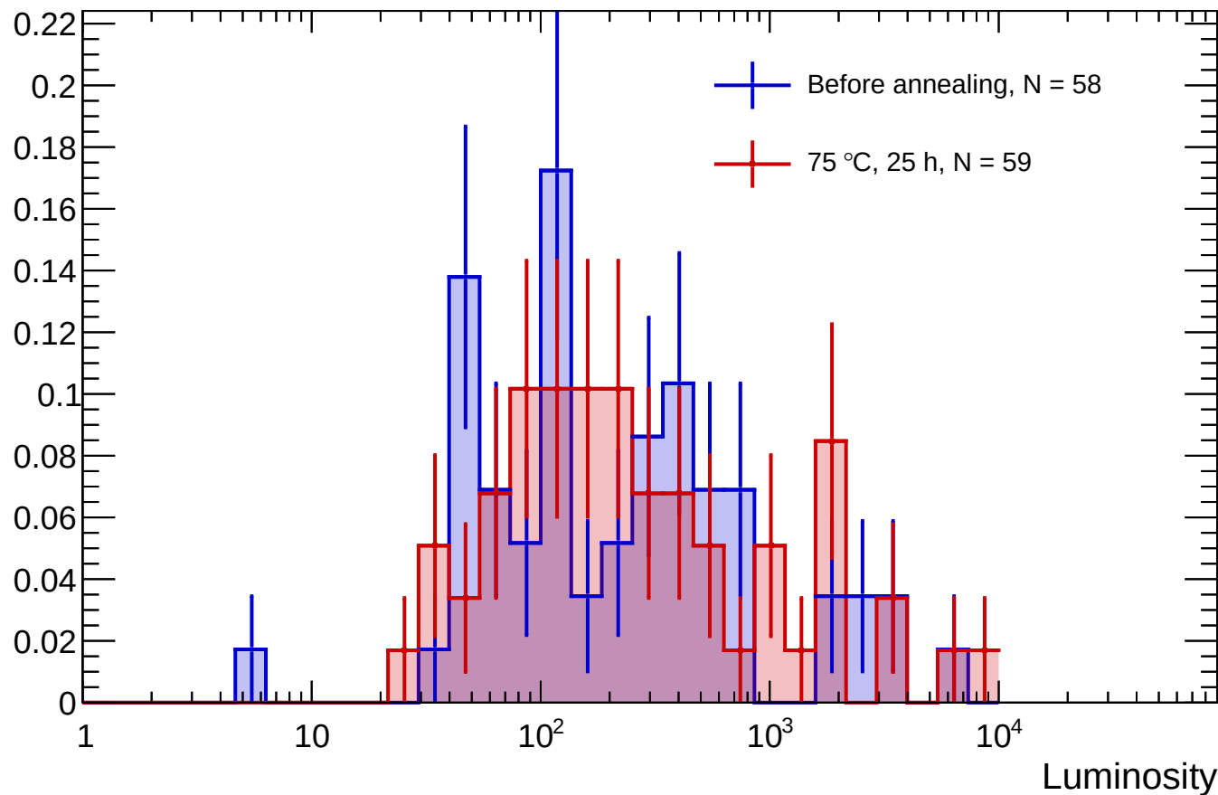
Sensor A1 - Before annealing vs 75 °C, 25 h luminosity distributions
