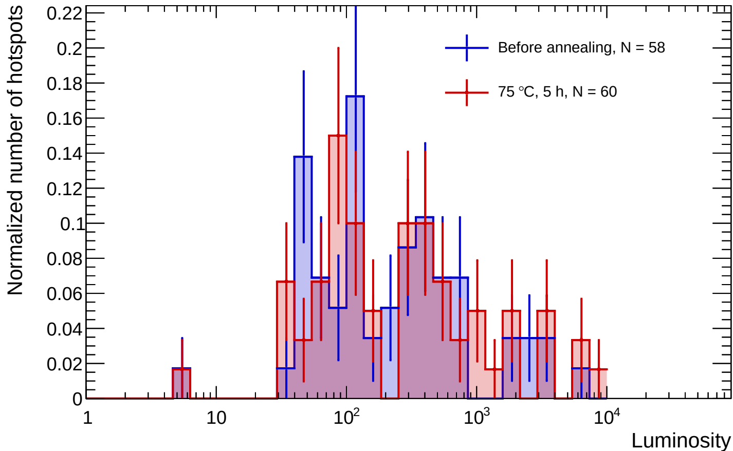
Sensor A1 - Before annealing vs 75 °C, 5 h luminosity distributions
