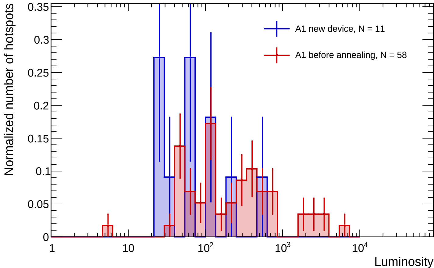
Sensor A1 - New device vs before annealing luminosity distributions
