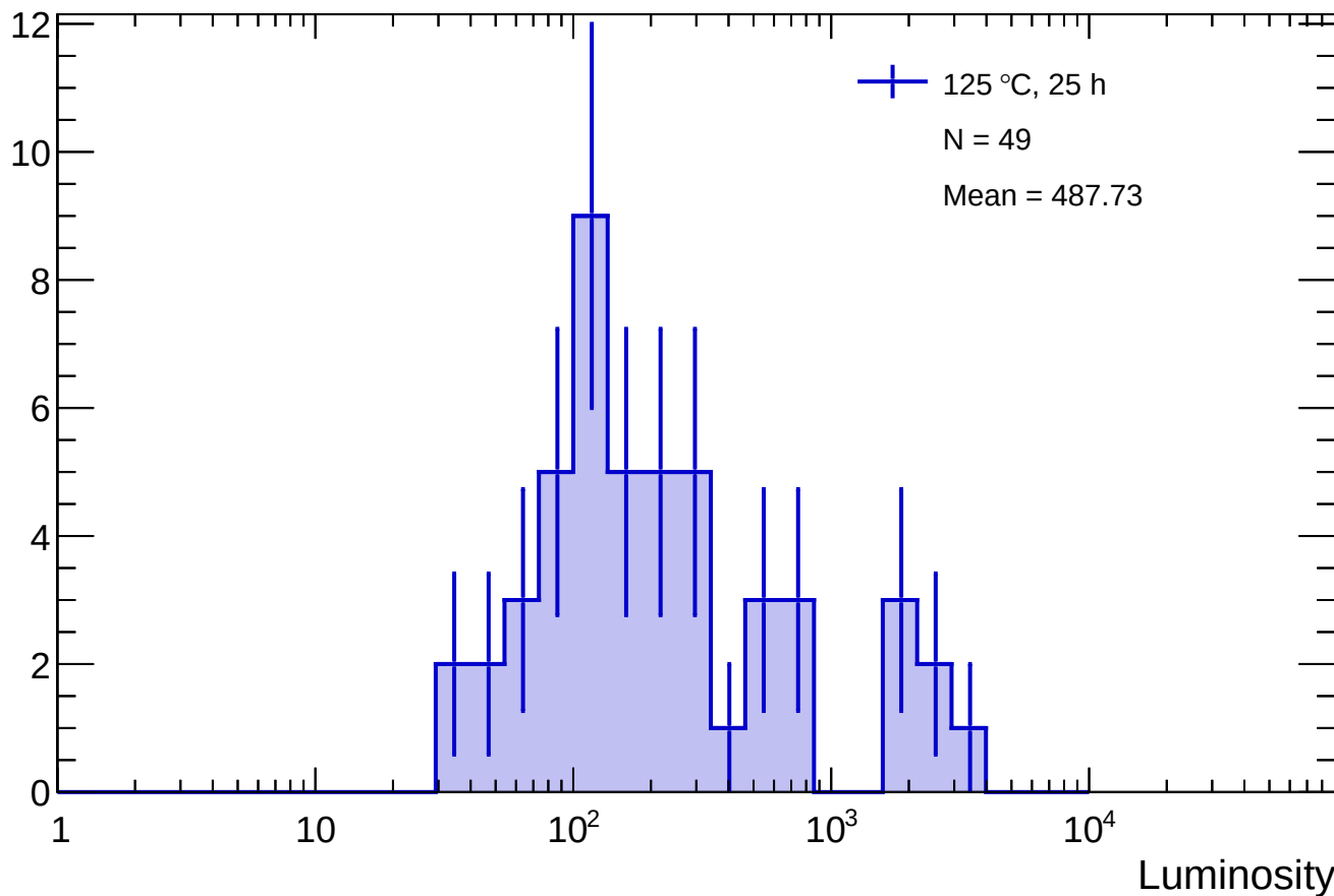
Sensor B1 - 125 °C, 25 h luminosity distribution
