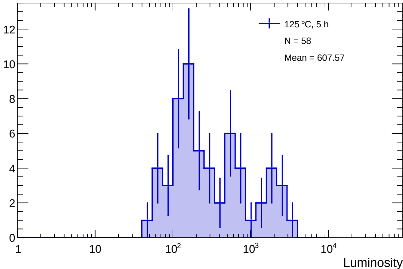
Sensor B1 - 125 °C, 5 h luminosity distribution
